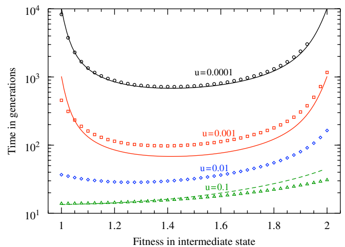
Fig. 2. Fixation times depending on the fitness in the intermediate state for a system with n = 2 . For small mutation rates ( u = 0.0001 ), the approximation from Eq. (5) (full lines) agrees well with numerical simulations (symbols). For larger u , the fixation times are no longer described well by the approximation in the limit of u \ll N^{-2} , but the minimum might still occur at the same point. For very large mutation rates ( u = 0.1 ), a deterministic limit of the process can be used to describe the fixation times (dashed line), see Appendix A. The dependence of the minimum on the mutation rate is shown in Fig. 3 (parameters N = 100 , r_0 = 1 , R = 2 , averages over 10^5 independent realizations of the process).
