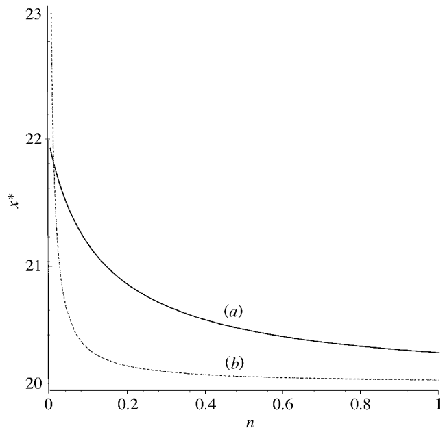
Figure 3. The influence of bystander effects ( n ) on the steady-state number of uninfected ( x ) CD4+ cells. The two curves represent two nonlinear immune functional responses: (a) the function \dot{z} = cy/(k + y) - bz includes proliferation and a density dependent rate of replication, while (b) only includes immune proliferation, \dot{z} = cy - bz . The parameter values used to generate this plot are \lambda = 0.5, d = 0.01, \beta = 0.001, a' = 0.1, a = 0.005, k = 0.05, p = 0.1, u = 0.01, b = 0.01, c = 0.001 .
