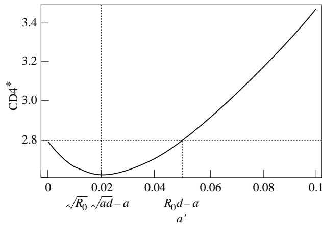
Figure 1. The reduction of CD4+ cells at equilibrium for different rates of CTL killing ( a' ). There is a minimum in the total number of CD4+ cells for increasing a' . Counterintuitively, it can be better to have no HIV-specific CTL response during infection. The parameter values used to generate this plot are \lambda = 0.1 , d = 0.001 , \beta = 0.05 , a = 0.05 , k = 0.01 , u = 0.01 .
