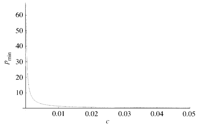
Figure 2. The minimum in total CD4+ cells ( p_{\min} ) as a function of immune responsiveness c . When the immune system is highly responsive, the minimum falls close to zero which implies that even weak or intermediate strengths of immune response can be worthwhile. The parameter values used to generate this plot are \lambda = 0.1 , d = 0.001 , \beta = 0.05 , a = 0.05 , k = 0.01 , b = 0.1 , u = 0.01 .
